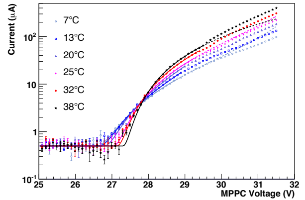
Fig. 6. Current vs voltage at different temperatures for the SensL SPMArray. The fit functions are overlaid over the data.
