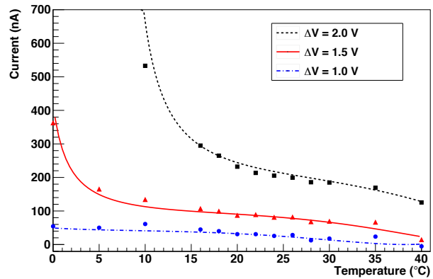
Fig. 10. Current vs temperature curves generated for 1 \times 4 \text{ mm}^2 MPPC 05 at 20^\circ\text{C} . The curves were calculated using previously extracted fit parameters. The plotted points represent measurements extracted from the I-V curves at each temperature.
