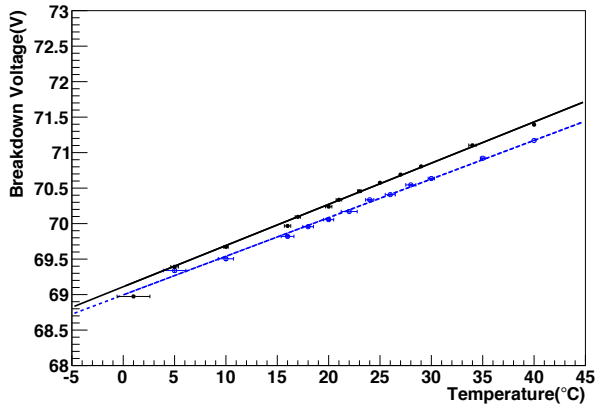
Fig. 7. Breakdown voltage versus temperature for 3x3 mm 2 MPPC 01 (filled circles, solid line) and 1x4 mm 2 MPPC 04 (open circles, dashed line).
