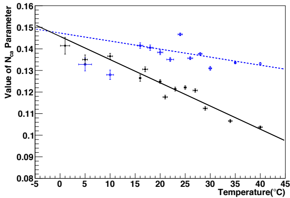
Fig. 8. Average number of correlated avalanches per parent avalanche ( N_{ca} parameter) versus temperature for 3 \times 3 \text{ mm}^2 MPPC 02 (filled circles, solid line) and 1 \times 4 \text{ mm}^2 MPPC 06 (open circles, dashed line).
